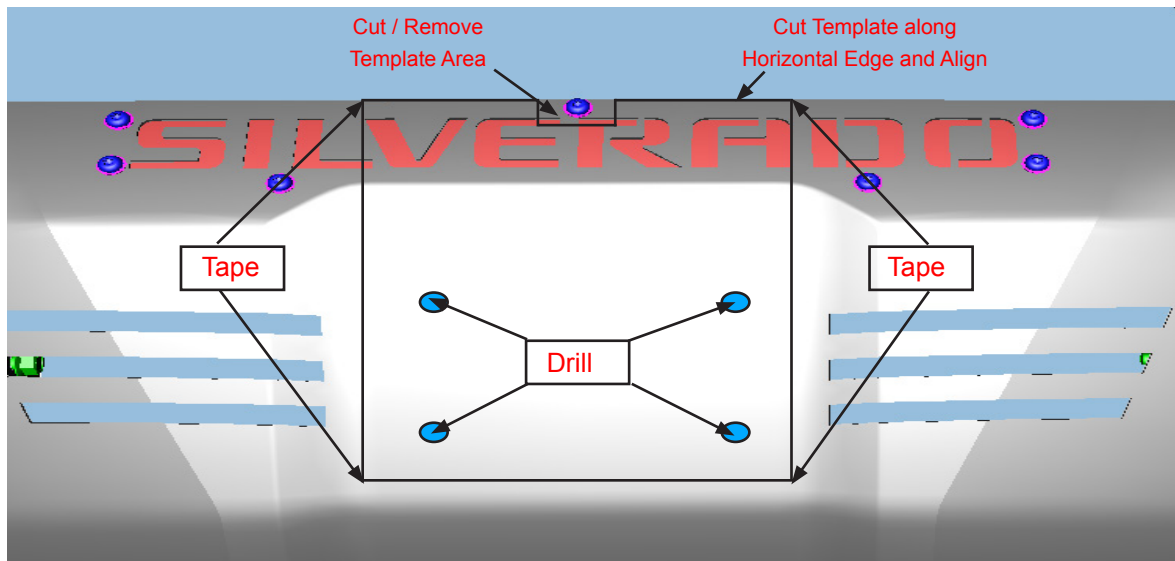
Figure 1. Align Drill Template to top edge as shown and securely tape in place before drilling.
